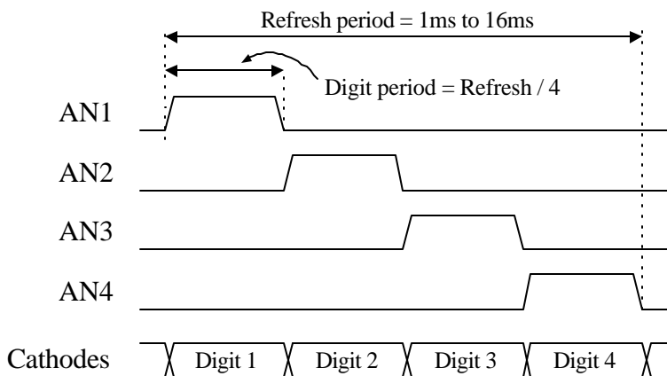
Seven segment display refresh signals and timings
